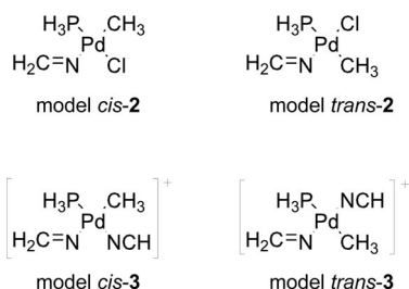
Scheme 3. Simplified models for theoretical calculations of complexes 2 and cations of compounds 3 .
