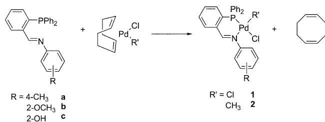
Scheme 1. Syntheses of complexes 1 and 2 .
