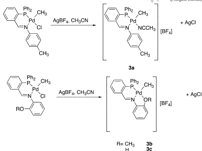
Scheme 2. Syntheses of compounds 3 .
