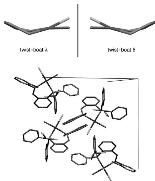
Figure 2. Fragments of the nonplanar chelating rings and packing in the unit cell (hydrogen atoms and solvent molecules omitted for clarity).
