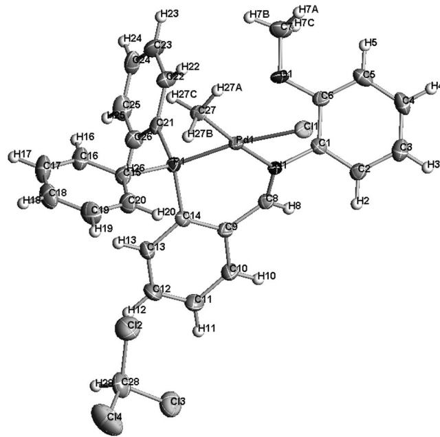
Figure 1. Structure of complex 2b . A chloroform molecule of crystallization is represented. Selected bond lengths and angles are summarized in Table 1.
