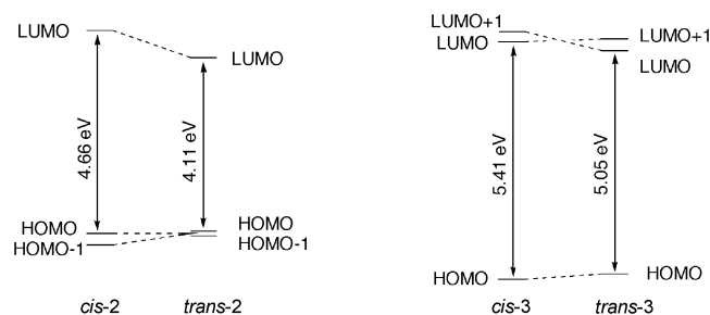
Figure 3. Relative energies of frontier orbitals in models 2 (left) and 3 (right).
